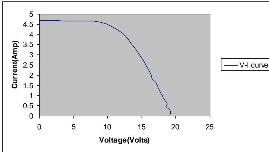
Fig.3. V-I Characteristics of 100W, 12V panel at 1.00pm
