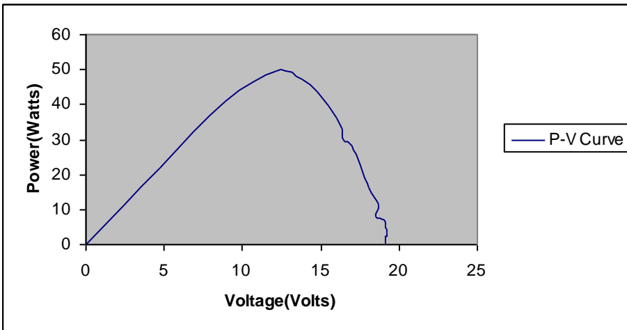
Fig. 2. P-V Characteristics for 1.00pm
