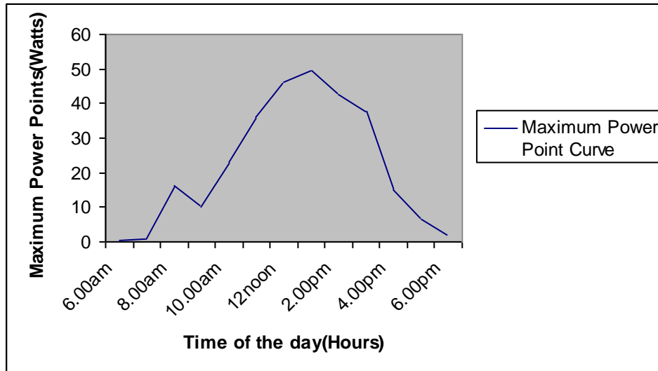
Fig.4. Maximum Power Point – Time characteristics
